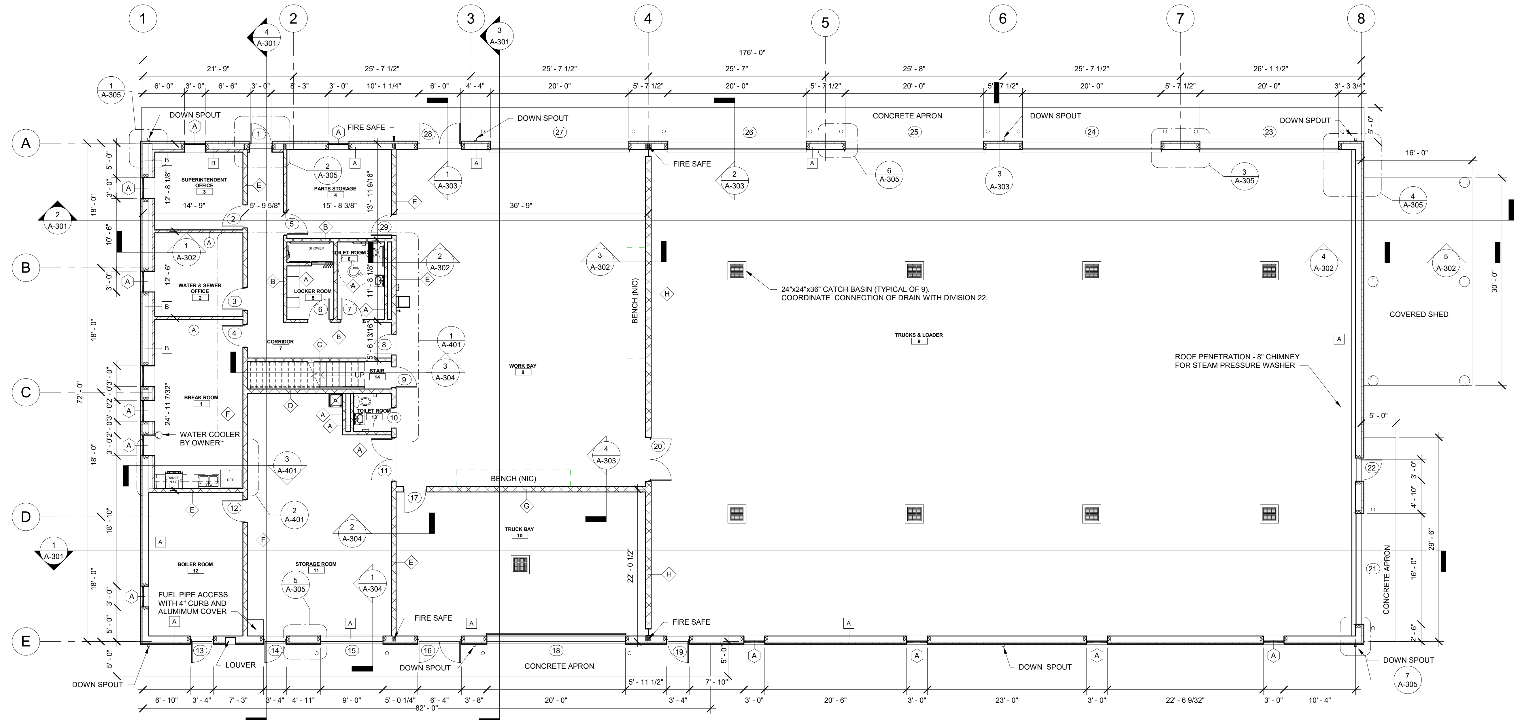
FIRST FLOOR PLAN SCALE: 1/8" = 1'-0"
